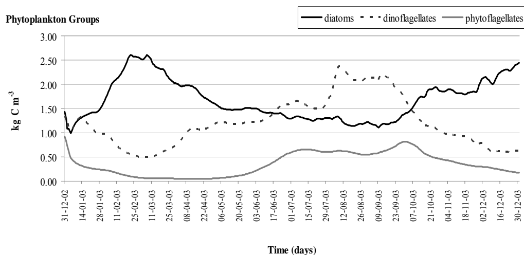
Fig. 2 - The modelled results of the three phytoplankton groups biomass ( \text{kg C m}^{-3} ).
