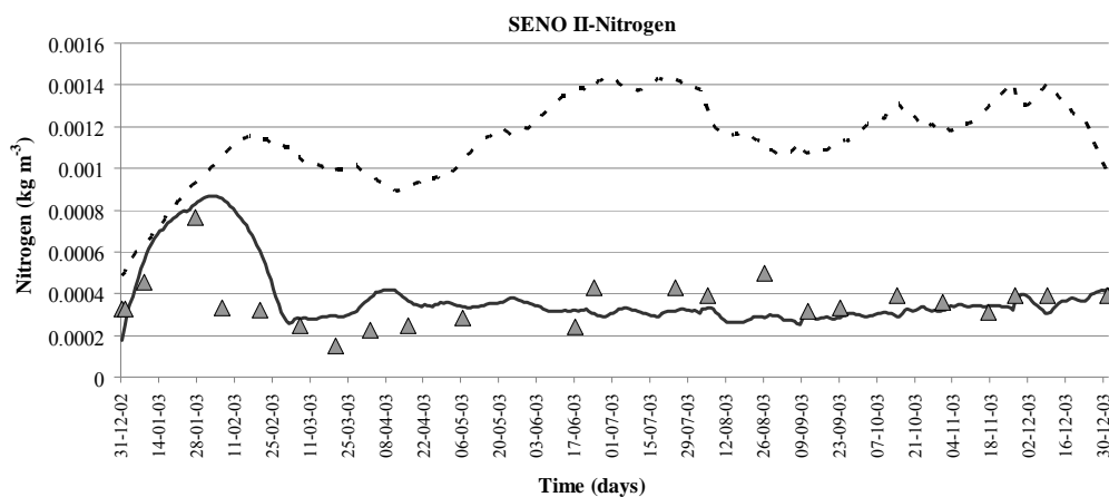
Fig. 1 - The simulated total nitrogen concentration at the surface (solid line) and bottom (dashed line) layers, compared to the experimental data collected at the surface (triangles).
