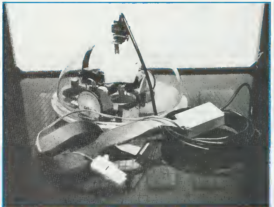
The Jessop Turtle. All the works can be seen beneath its perspex dome
