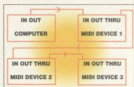
MIDI connections
