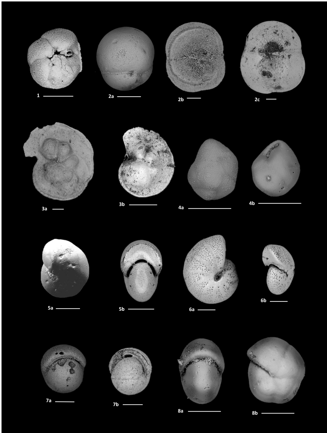
Figure 7. Scale bar is 100 \mu\text{m} . (1) Gavelinopsis lobatulus , ODP Hole 752A, 3H-5, 62–67 cm: umbilical view. (2a–c) Sphaeroidina bulloides , (2a) ODP Hole 752A, 8H-1, 100–105 cm: side view. (2b) ODP Hole 1139A, 8R-1, 45–49 cm: apertural side view. (2c) ODP Hole 1168A, 26X-2, 73–77 cm: apertural side view. (3a–b) Laticarinina pauperata , (3a) ODP Hole 752A, 7H-2, 73–78 cm: umbilical view. (3b) ODP Hole 1139A, 18R-1, 96–100 cm: umbilical view. (4a–b) Epistominella exigua , ODP Hole 1168A, 36X-6, 62.5–66.5 cm: (4a) spiral view; (4b) umbilical view. (5a–b) Astrononion umbilicatum , ODP Hole 1139A, (5a) 19R-2, 60.5–64.5 cm: umbilical view. (5b) 17R-3, 91–95 cm: edge view. (6a–b) Melonis barleeanus , ODP Hole 1139A, (6a) 4R-2, 105–109 cm: umbilical? view. (6b) 19R-2, 60.5–64.5 cm: edge view. (7a–b) Pullenia bulloides , (7a) ODP Hole 752A, 9H-5, 65–70 cm: edge view. (7b) ODP Hole 1139A, 16R-2, 55–59 cm: edge view. (8a–b) Pullenia quinqueloba , ODP Hole 1168A, 35X-1, 65–69 cm: (8a) edge view; (8b) umbilical view.
