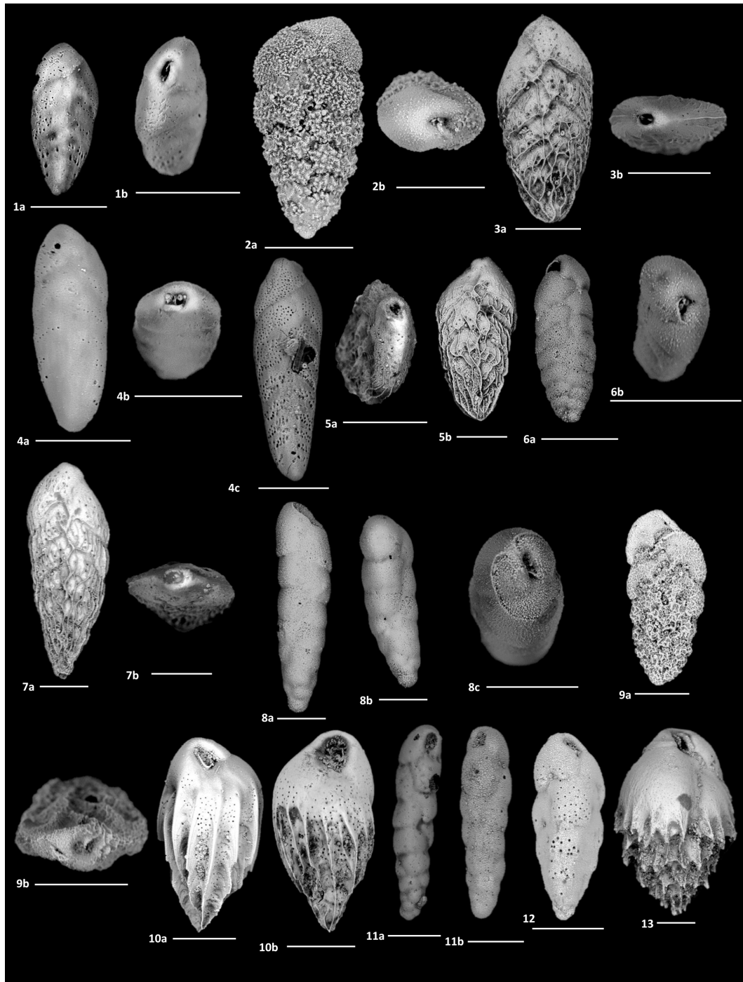
Figure 3. Scale bar is 100 \mu\text{m} . (1a–b) Bolivina dilatata , ODP Hole 1168A, 37X-6, 75–79 cm: (1a) side view; (1b) apertural view. (2a–b) Bolivina huneri , ODP Hole 752A, 10H-5, 77–81 cm. (2a) side view; (2b) apertural view. (3a–b) Bolivina reticulata , ODP Hole 1168A, 15X-2, 76–80 cm: (3a) side view; (3b) apertural view. (4a–b) Bolivina sp. 3, ODP Hole 1168A, (4a–b) 26X-2, 73–77 cm: (4a) side view; (4b) apertural view. (4c) 37X-6, 75–79 cm: side view. (5a–b) Bolivina cf. reticulata , ODP Hole 752A, (5a) 5H-1, 65–70 cm: apertural view. (5b) 3H-5, 62–67 cm: side view. (6a–b) Bolivina sp. 9, ODP Hole 752A, 9H-2, 104–109 cm: (6a) side view; (6b) apertural view. (7a–b) Bolivina viennensis , ODP Hole 752A, 5H-1, 65–70 cm: (7a) side view; (7b) apertural view. (8a–c) Bolivinelina cf. B. translucens , ODP Hole 752A, 3H-1, 50–55 cm: (8a–b) side view; (8c) apertural view. (9a–b) Abditodentrix pseudothalmanni , ODP Hole 1139A, 19R-2, 60.5–64.5 cm: (9a) side view; (9b) apertural view. (10a–b) Bulimina truncana , (10a) ODP Hole 752A, 9H-5, 65–70 cm: lateral view. (10b) ODP Hole 1168A, 37X-6, 75–79 cm: apertural side view. (11a–b) Bulimina cf. B. elongata , (11a) ODP Hole 1168A, 23X-3, 74–78 cm: apertural side view. (11b) ODP Hole 1139A, 18R-1, 96–100 cm: apertural side view. (12) Bulimina gibba , ODP Hole 1139A, 19R-2, 60.5–64.5 cm: lateral view. (13) Bulimina striata , ODP Hole 752A, 5H-1, 65–70 cm: apertural side view.
