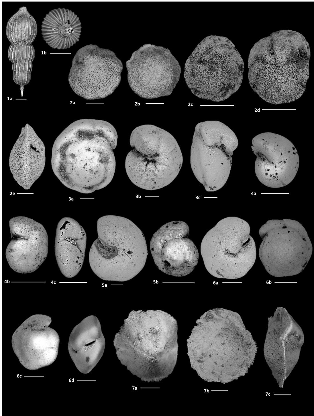
Figure 6. Scale bar is 100 \mu\text{m} . (1a–b) Amphicoryna scalaris , ODP Hole 752A, (1a) 10H-5, 77–81 cm: side view. (1b) 8H-1, 100–105 cm: apertural view. (2a–e) Nuttallides umbonifera , (2a, e) ODP Hole 752A, 4H-5, 64–69 cm: (2a) umbilical view; (2e) edge view. (2b) ODP Hole 752A, 9H-5, 65–70 cm: spiral view. (2c) ODP Hole 1168A, 13X-1, 40–44 cm: spiral view. (2d) ODP Hole 1168A, 14X-4, 45–49 cm: umbilical view. (3a–c) Gyroidinoides soldanii , ODP Hole 1139A, 3R-4, 32–36 cm: (3a) spiral view; (3b) umbilical view; (3c) edge view. (4a–c) Gyroidinoides sp. 1, ODP Hole 1139A, (4a, c) 19R-2, 60.5–64.5 cm: (4a) spiral view; (4c) edge view. (4b) 17R-3, 91–95 cm: umbilical view. (5a–b) Gyroidinoides sp. 2, (5a) ODP Hole 1168A, 32X-4, 80–84 cm: umbilical view. (5b) ODP Hole 1139A, 15R-4, 41–45 cm: spiral view. (6a–d) Oridorsalis umbonatus , (6a–b) ODP Hole 1168A, 8H-1, 100–104 cm: (6a) umbilical view; (6b) spiral view. (6c) ODP Hole 752A, 5H-1, 65–70 cm: spiral view. (6d) ODP Hole 1168A, 8H-1, 100–104 cm: edge view. (7a–c) Osangularia culter , ODP Hole 1168A, 28X-3, 75–79 cm: (7a) umbilical view; (7b) spiral view; (7c) edge view.
