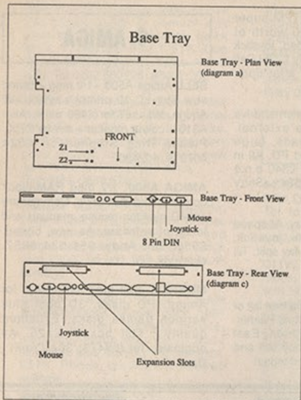
• The Base Tray – Plan view (top), Front view (centre), Rear view (bottom).
