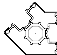
2-WAY 135° PANEL CONNECTOR (Plan View)
