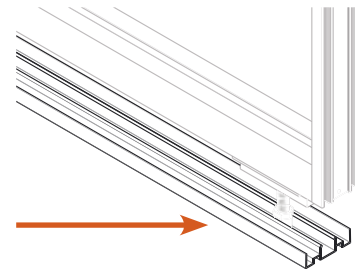
FLOOR RUNNER for 4" and 6" VINYL BASE (Specified and shipped separately)
