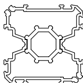
4-WAY PANEL CONNECTOR (Plan View)
