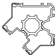
3-WAY PANEL CONNECTOR 90°/135° (Plan View)
