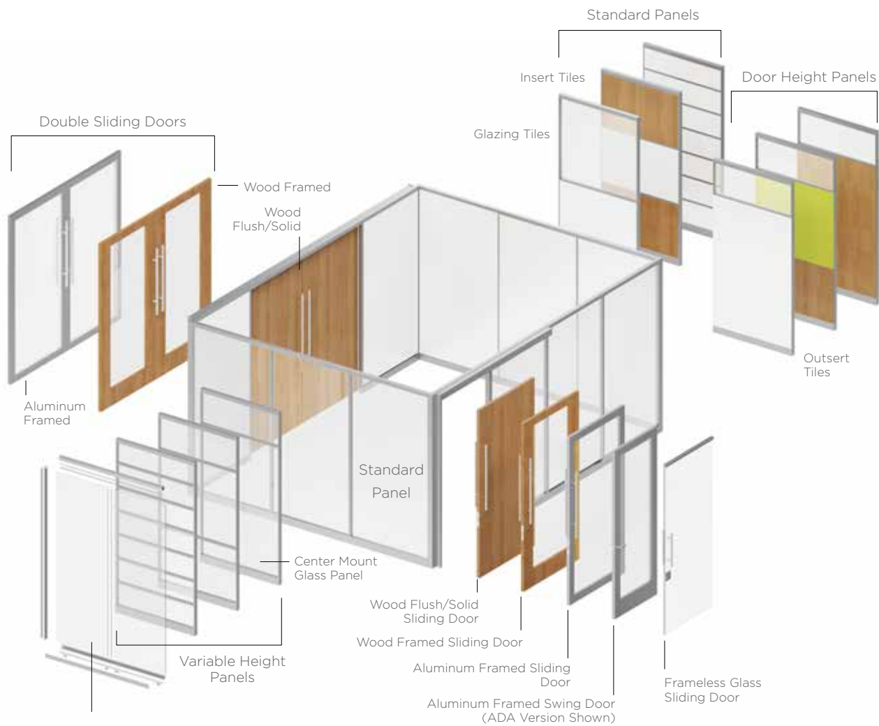
Frameless Glass Wall, a kit of parts including Glass Inserts and Framing Elements
