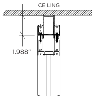
PANEL AS SPECIFIED WITH ONE PANEL EXTENDER
