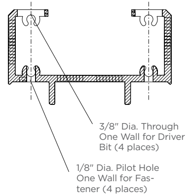
PANEL EXTENDER part # 395796 (Profile View)
