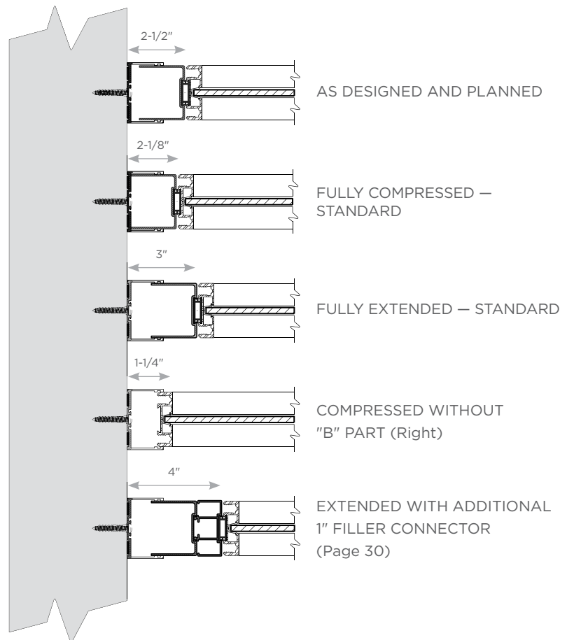
ADJUSTABLE WALL START ADJUSTMENT RANGE
