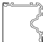
90° CORNER CONNECTOR (Plan View)
