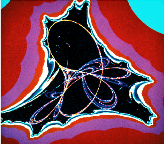
Tinkerbell Attractor and basin of attraction
