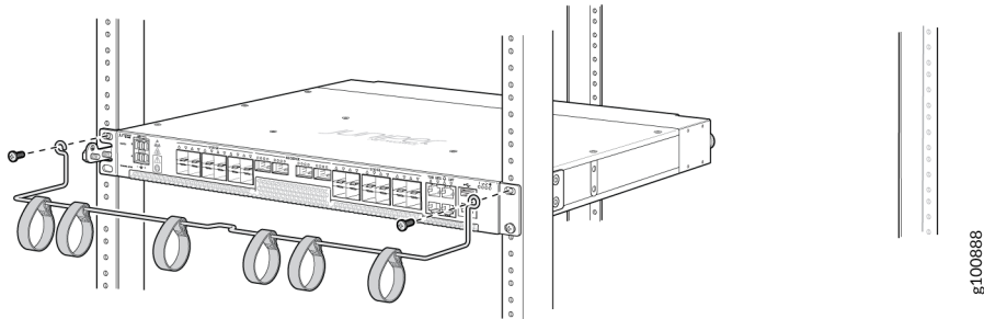
Figure 12: Install the Cable Bar
