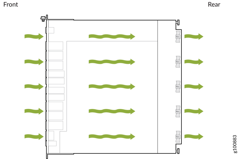
Figure 7: Airflow Through the ACX710 Chassis
