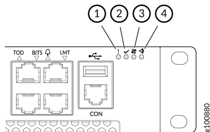
Figure 5: Chassis Status LEDs on an ACX710 Router
