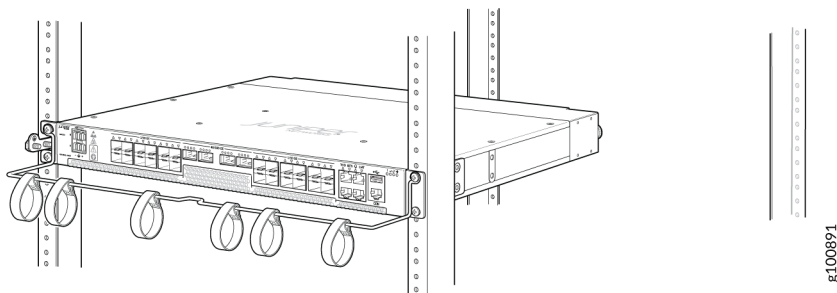
Figure 13: ACX710 Router Installed in a Four-Post Rack
