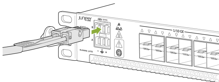
Figure 18: Connect a DC Power Cord to an ACX710 Router
