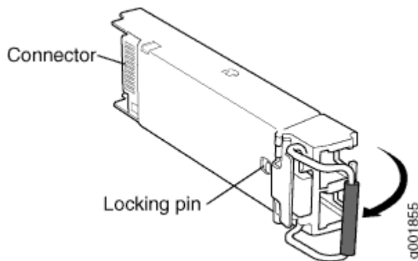
Figure 25: Small Form-Factor Pluggable (SFP) Transceiver
