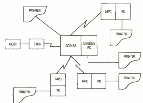
Cluster Controller
