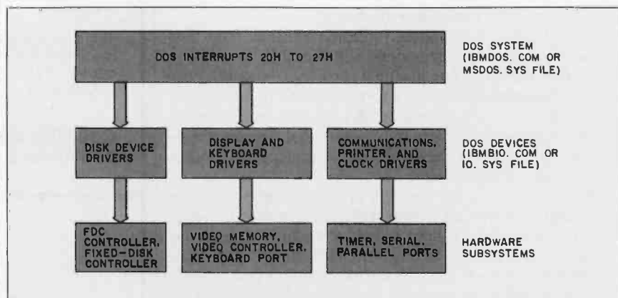
Figure 1: An architectural model of the IBM PC and XT.
